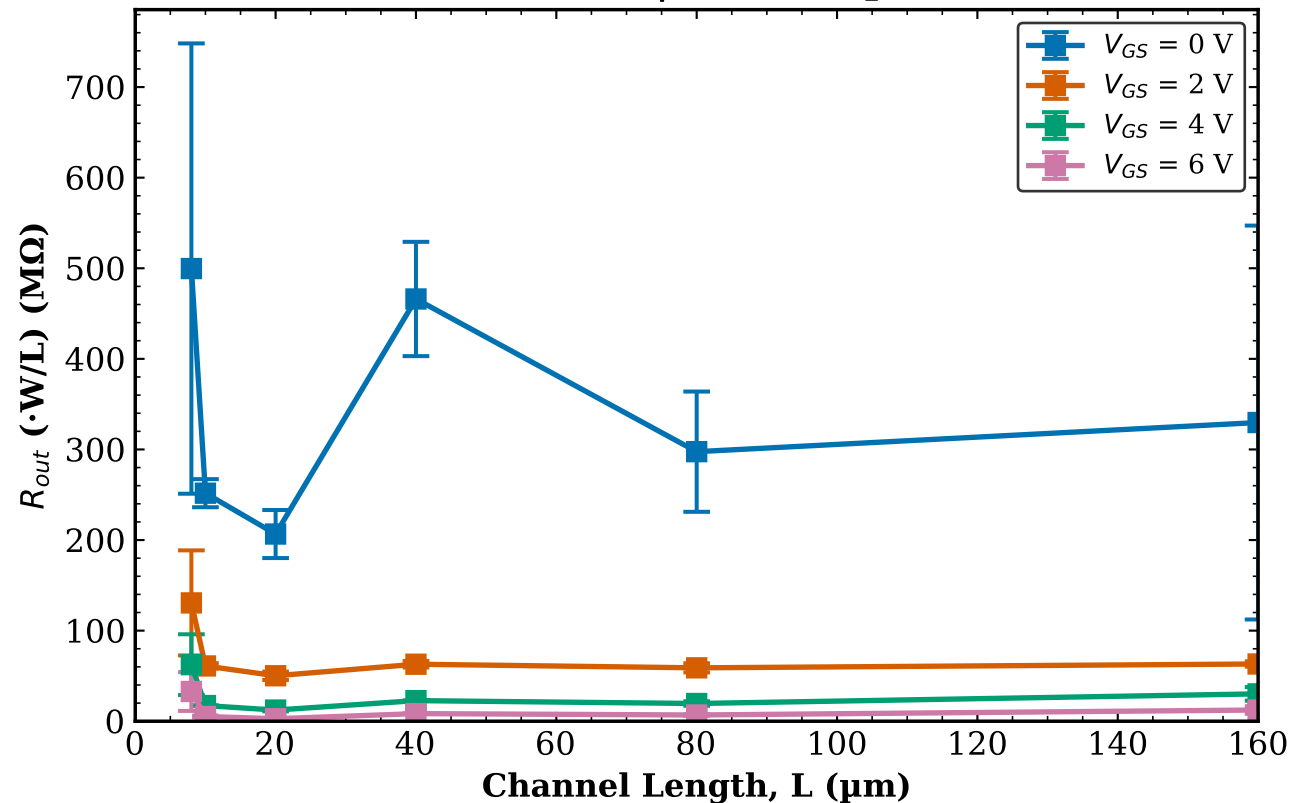
TFT1 Combined (Tr. 1 & 2) R_{out} vs L | W = 10\text{ }\mu\text{m}
